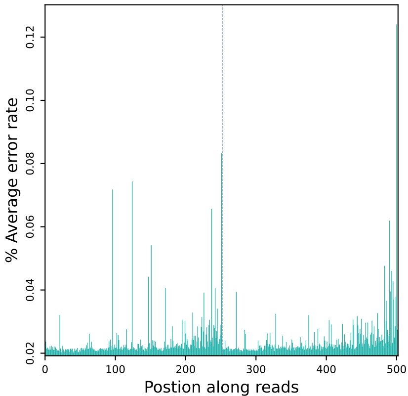
Error rate distribution along reads (R10608)
